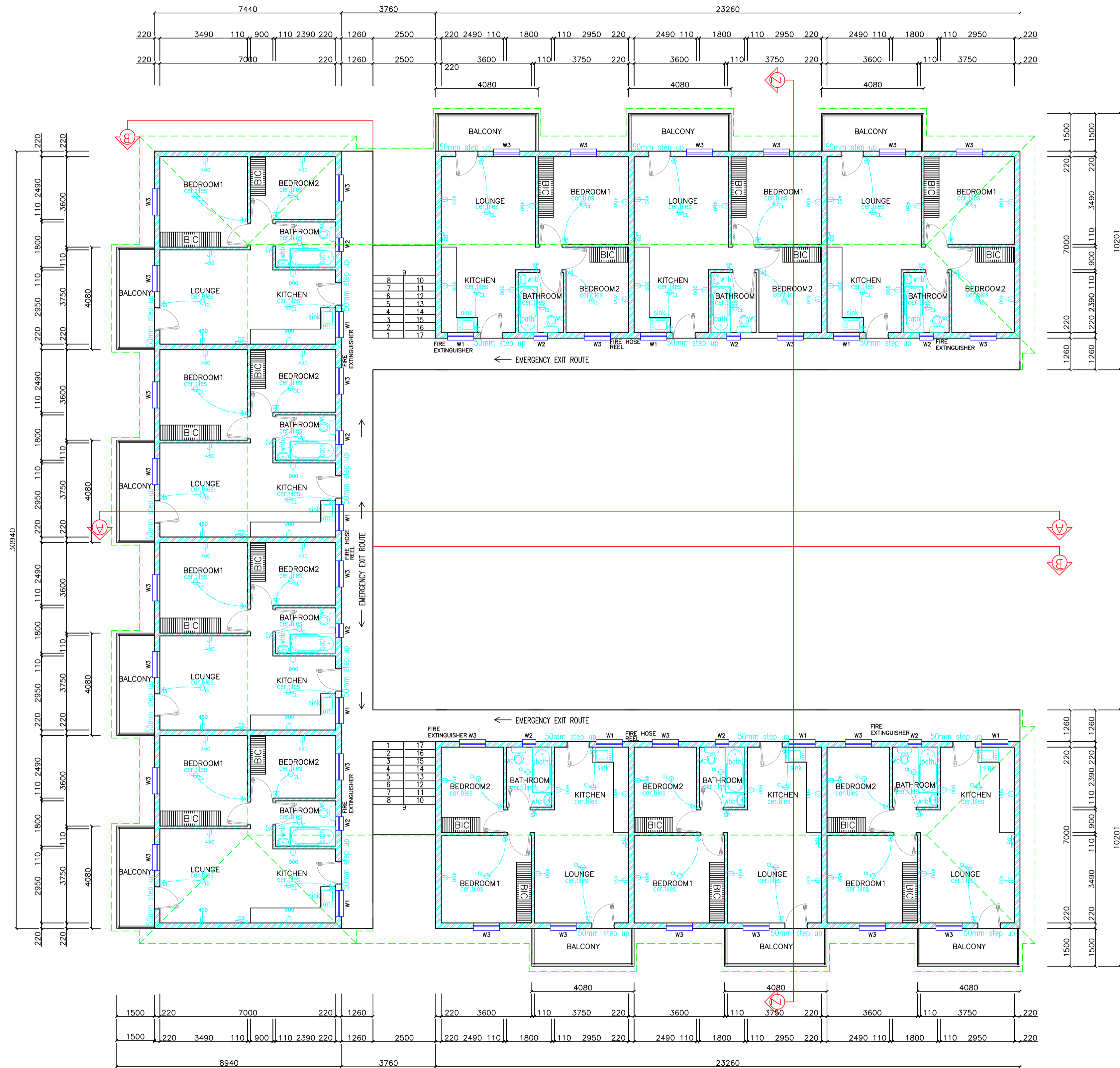
FIRST FLOOR PLAN SCALE 1:100
